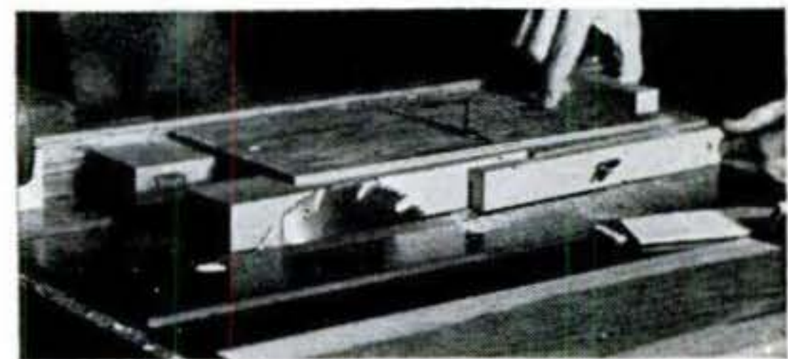
THE QUICK-SETTING JIG does a production run of model-airplane wings. Stop is clamped to fence.
